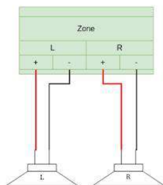
Standard Wiring – 2 speakers (L+R) run in parallel per zone
